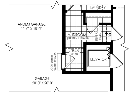
Partial Opt. Ground Floor with Elevator Elevation A & B
