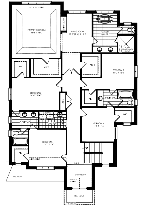
Optional 5 Bedroom Layout Elevation A
